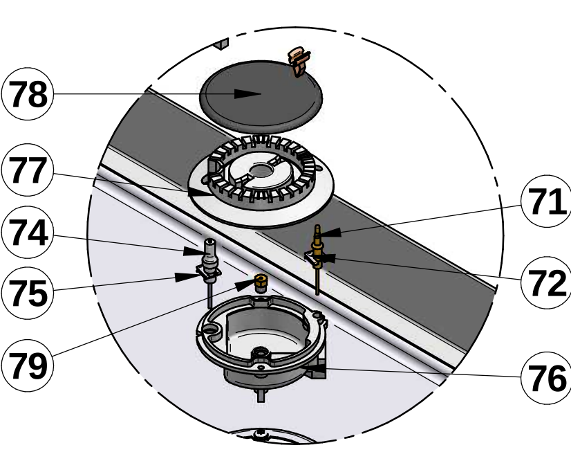
DETAIL F
