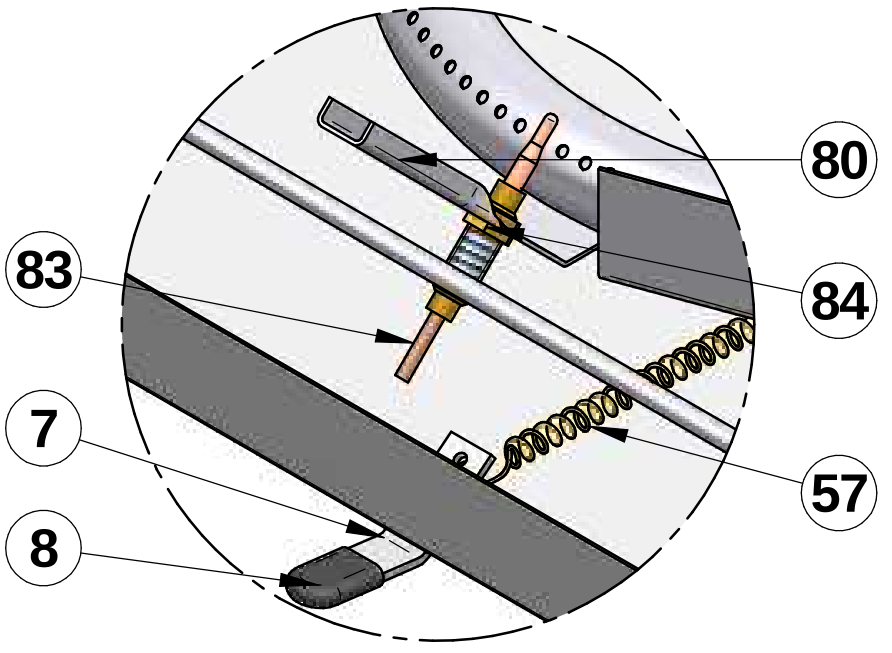
DETAIL D
